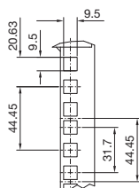
Detail X
