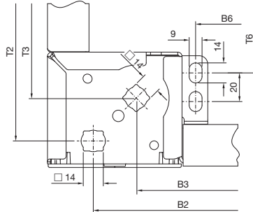
Base/plinth corner pieces with base/plinth trim panels, front and rear
